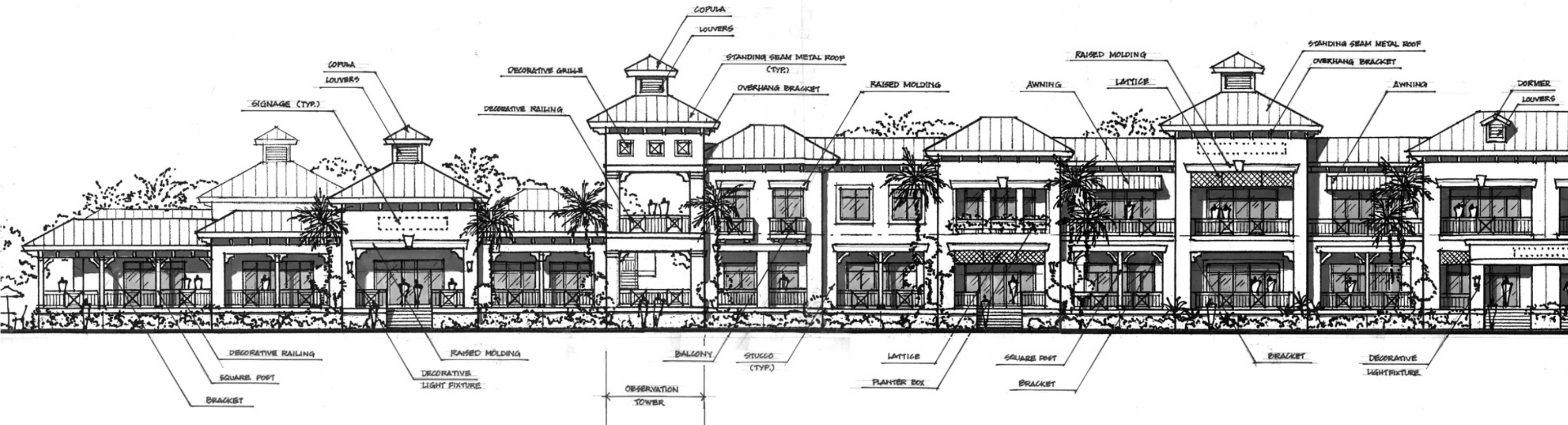
East Elevation
